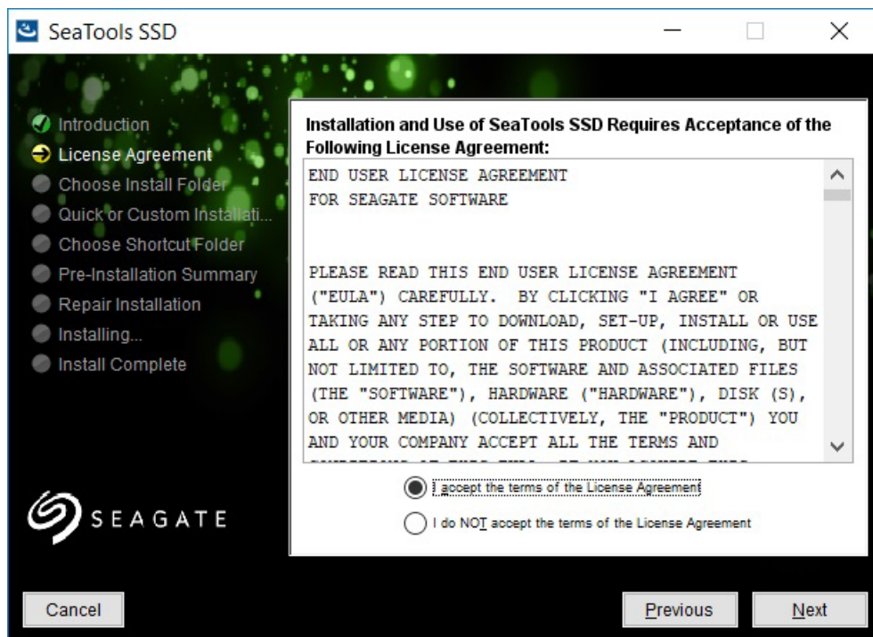
Figure 2 Installation—License Agreement
