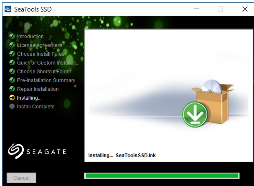
Figure 5 Installation Progress
