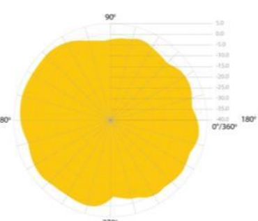
5GHz 2D Radiation Pattern@ Vertical
