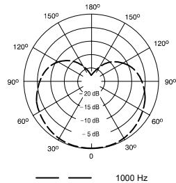
典型指向性图样
